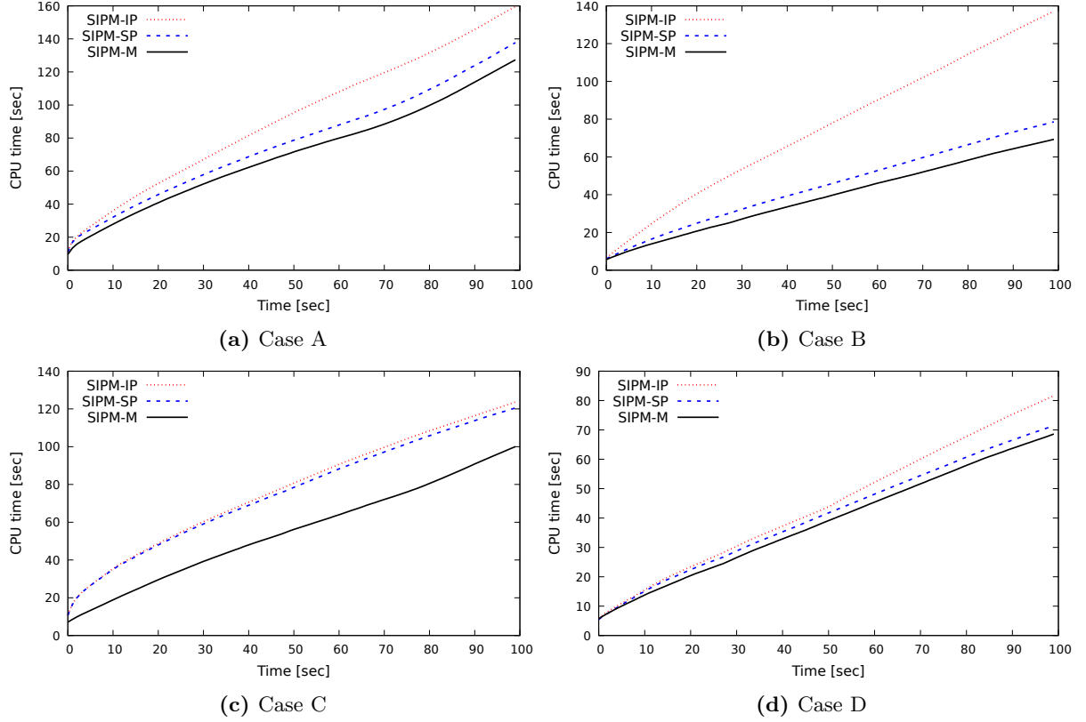
Figure 13. CPU time as a function of simulation time for unsteady conjugate natural convection in three square enclosures with three solids (state A to D) solved by classic partitioned, proposed partitioned, and proposed monolithic solvers
