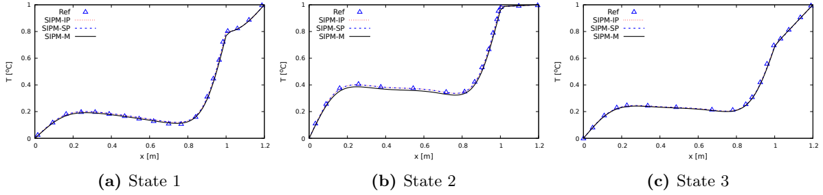
Figure 7. Temperature profile for three states of the unsteady conjugate natural convection in a single square enclosure at y = 0.5 m and t = 0.07 s given by three solvers (SIPM-IP or the classic partitioned, SIPM-SP or the proposed partitioned, SIPM-M or the proposed monolithic) and literature [38].
