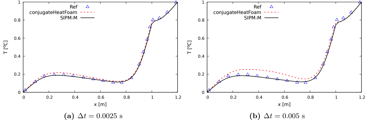
Figure 8. Temperature profile for state 1 of the unsteady conjugate natural convection in a single square enclosure at y = 0.5 m and t = 0.07 s given by proposed monolithic (SIPM-M), OpenFOAM® (conjugateHeatFoam), and literature
