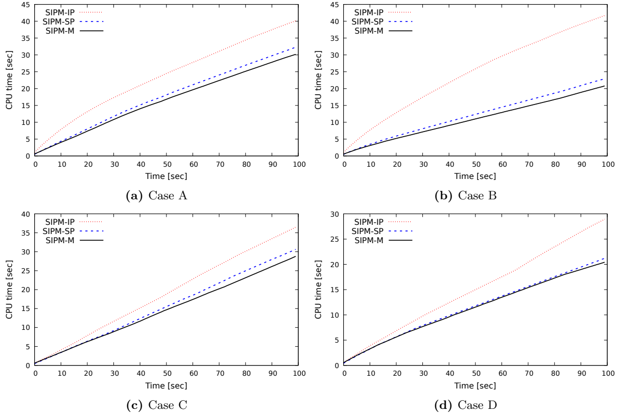
Figure 9. Cumulative CPU time as a function of simulation time for unsteady conjugate natural convection in a single square enclosure with a single solid (state A to D) solved by classic partitioned (SIPM-IP), proposed partitioned (SIPM-SP), and proposed monolithic solvers (SIPM-M)
