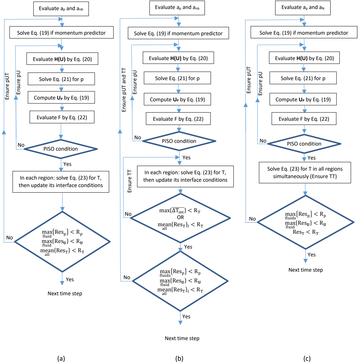
Figure 4. Flowchart of the algorithms for each time step (a) classic partitioned algorithm, SIPM-IP (b) proposed partitioned, SIPM-SP (c) proposed monolithic algorithm, SIPM-M
