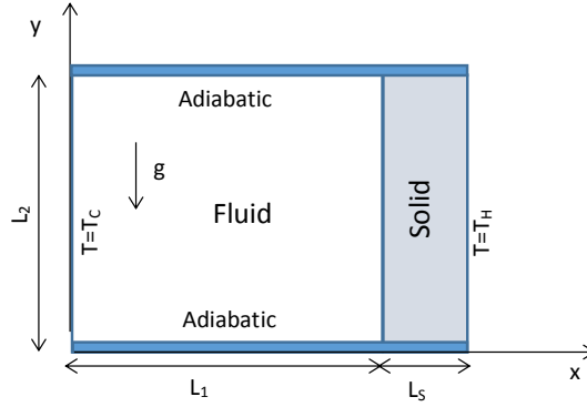
Figure 5. Conjugate natural convection in a single square enclosure
