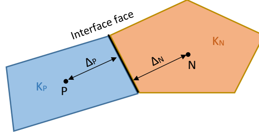
Figure 3. Owner (blue) and neighbour (orange) cells at both sides of the shared interface faces
