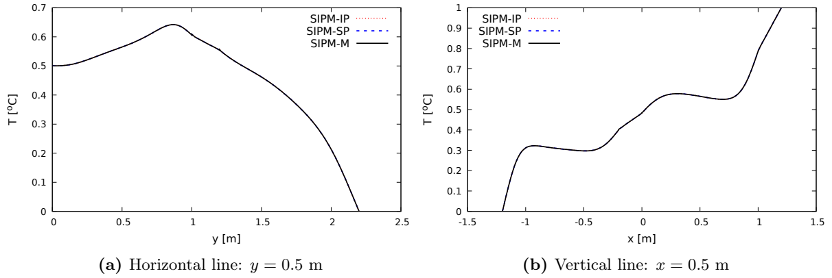
Figure 12. Temperature profile at lines y = 0.5 m and x = 0.5 m given by three proposed solvers for unsteady conjugate natural convection in three square enclosures with three walls (state A) at t = 0.07 s
