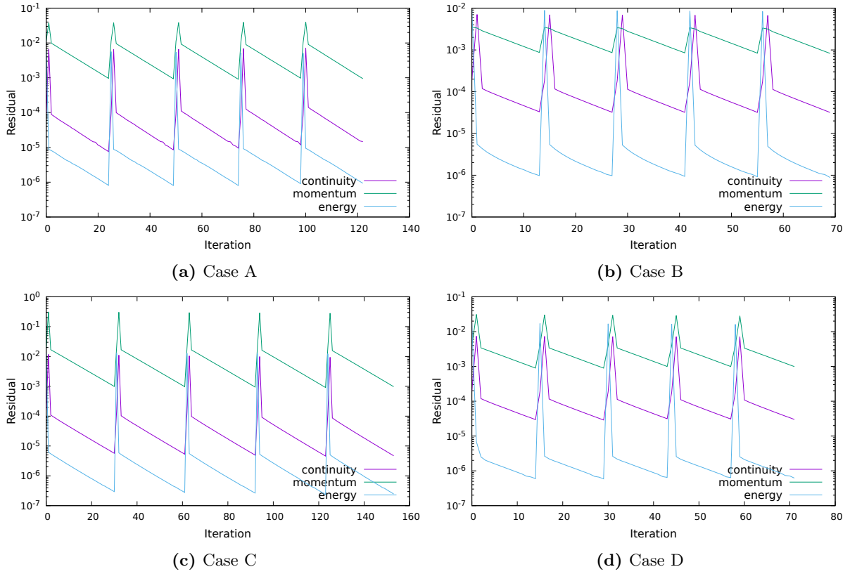
Figure 14. Residual convergence history over five consecutive time steps for unsteady conjugate natural convection in three square enclosures with three solids (states A to D), solved by the proposed partitioned solver without utilizing the momentum predictor
