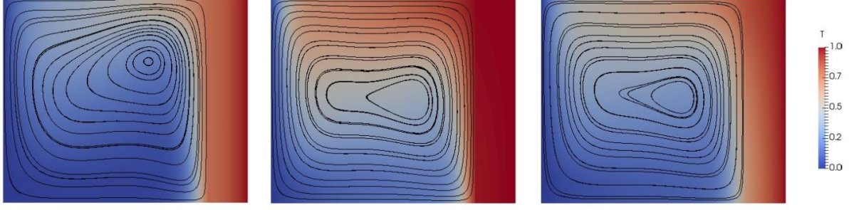
Figure 6. Contour of temperature and streamline for three states of the unsteady conjugate natural convection in a single square enclosure at t = 0.07 s
