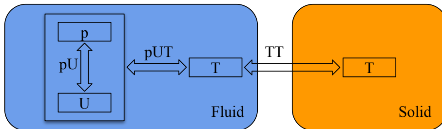
Figure 1. Three types of coupling in the equations of conjugate heat transfer
