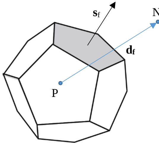
Figure 2. Control volume P, its neighbour N, and the relevant cell-face parameters
