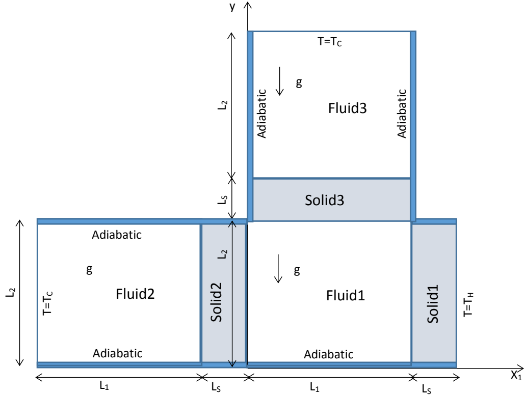
Figure 10. Schematic of unsteady conjugate natural convection in three square enclosures with three solid walls
